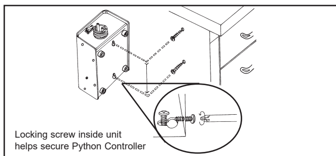
Figure 7. Installing controller to bench.
