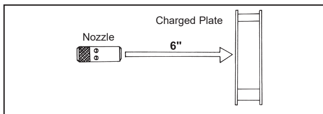
Figure 9. EOS/ESD S-3.1 decay time test set up.
